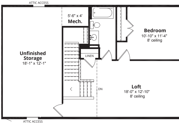
SECOND FLOOR 536 finished sq. ft.
