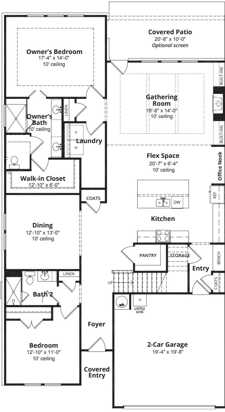
FIRST FLOOR 2,017 finished sq. ft.
