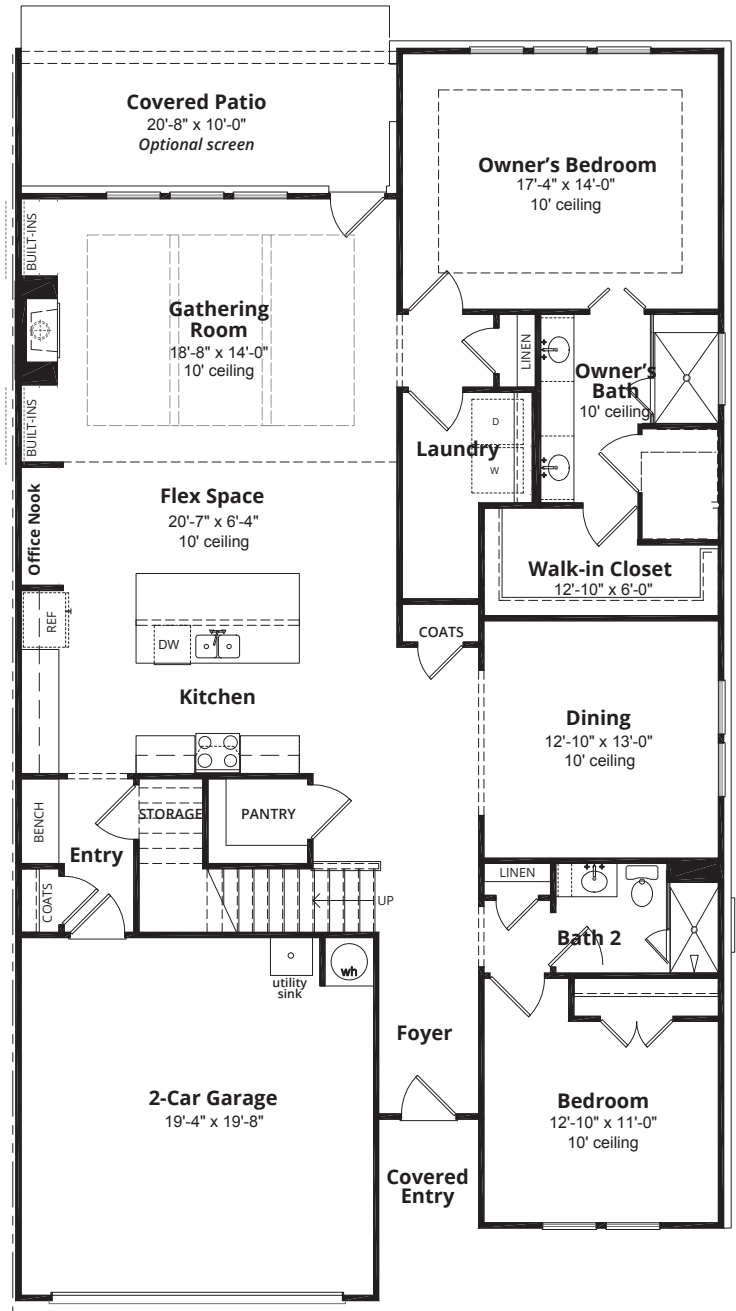
FIRST FLOOR 2,017 finished sq. ft.
